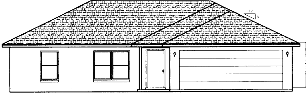
FRONT ELEVATION
